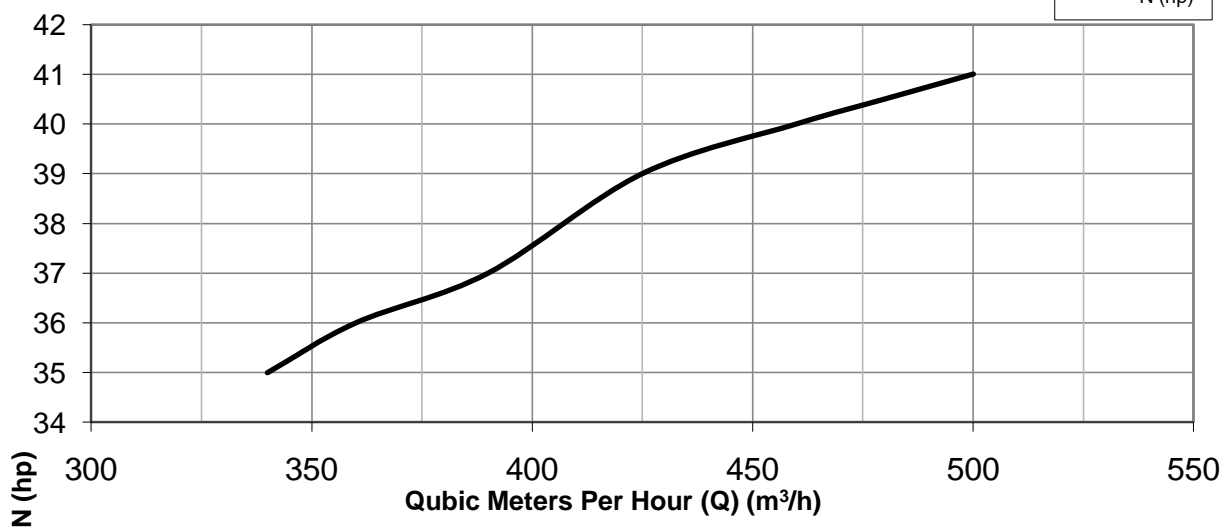
Brake Horse Power (hp) Vs Q
