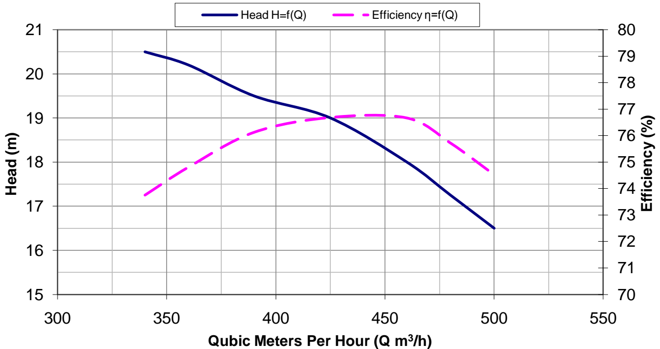
Performance Curve For Stage 14KHKB (1490 RPM)
