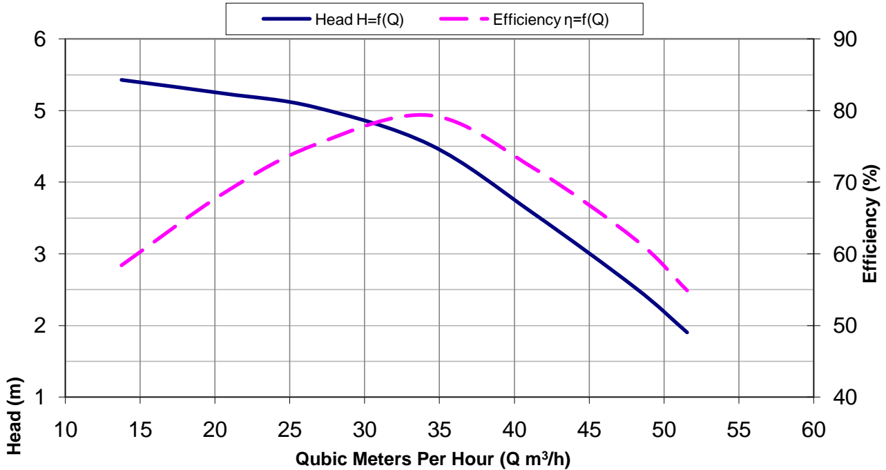
Performance Curve For Stage 7HKB (1490RPM)
