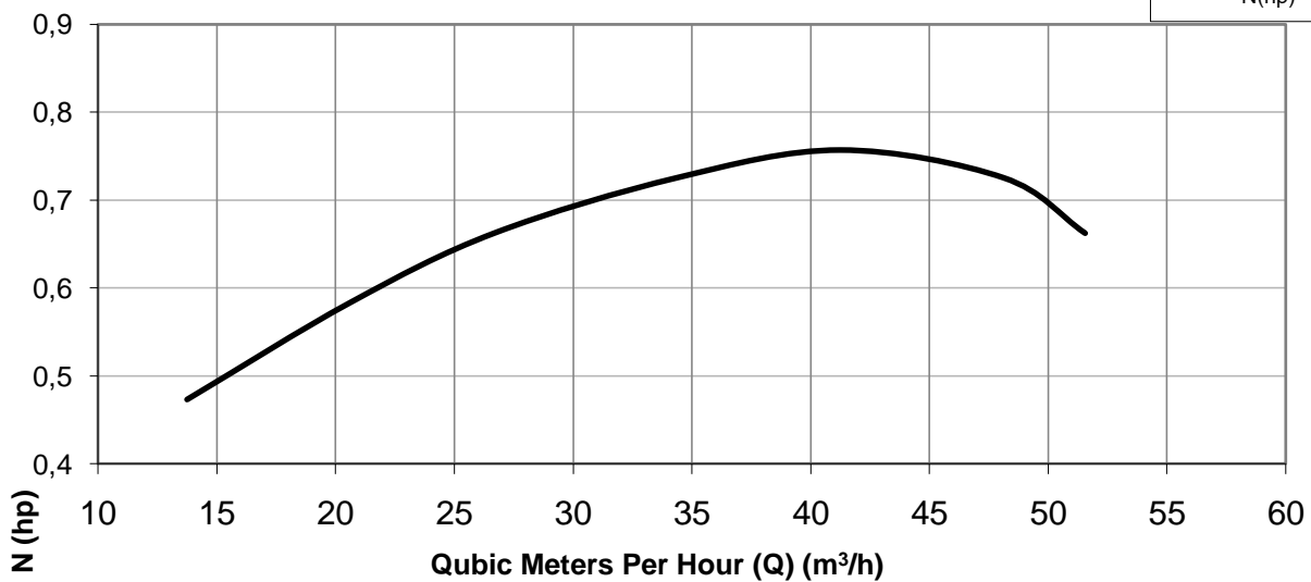
Brake Horse Power (hp) Vs Q
