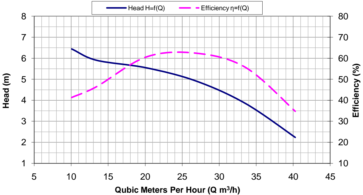
Performance Curve For Stage 4HKB (2960RPM)
